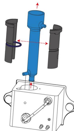
16 mm Reaction Cell Positioned Over the Chamber with the Adapter
