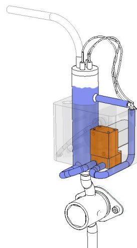
Mixing Pump Position with Cell
