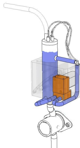
26 mm Reaction Cell with the overflow tube attached and mixing in progress
