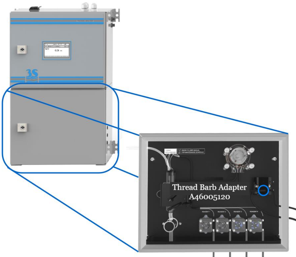
(1) Thread Barb Adapter (Hose Barb 1/8") for two inlet liquids
