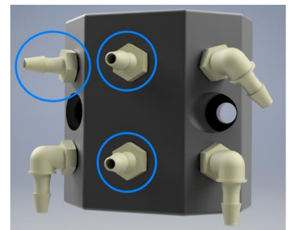
(3) Thread Barb Adapters (Hose Barb 1/8") for three inlet liquids
