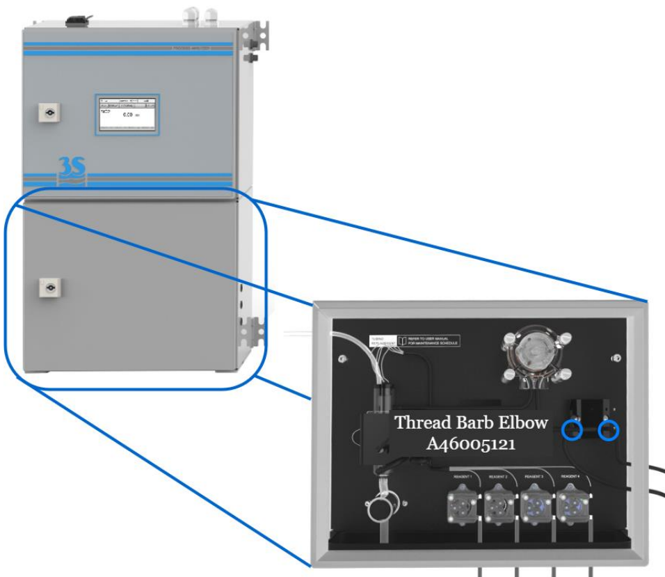
(2) Thread Barb Elbows (Hose Barb 1/8") for two inlet liquids
