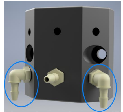
(2) Thread Barb Elbows (Hose Barb 1/8") for two inlet liquids
