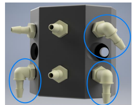
(3) Thread Barb Elbows (Hose Barb 1/8") for three inlet liquids
